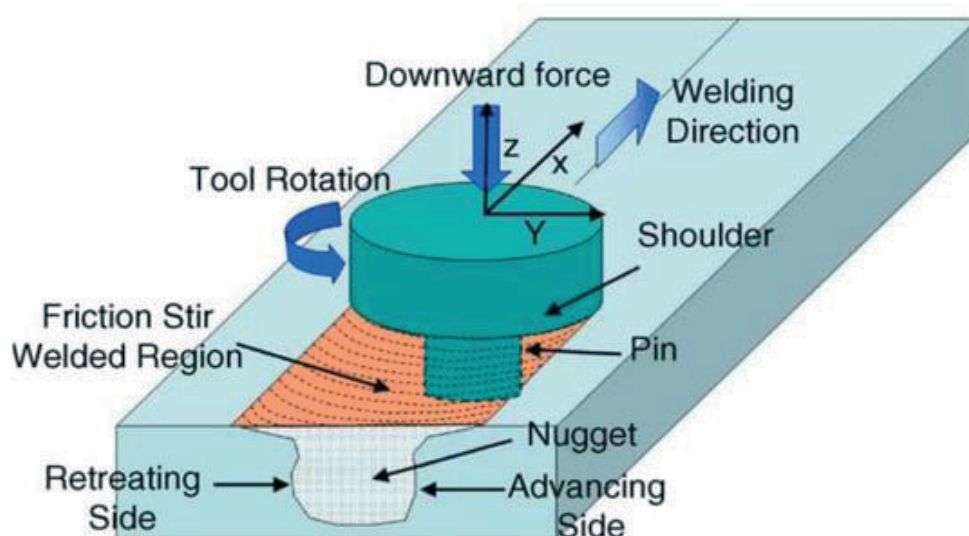
FIGURE 1. FSW detailed view [17]
