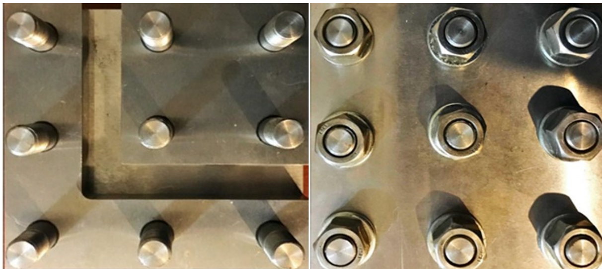
FIGURE 2. Equal channel angular compression mold used in the experiments in open and closed states, top view
