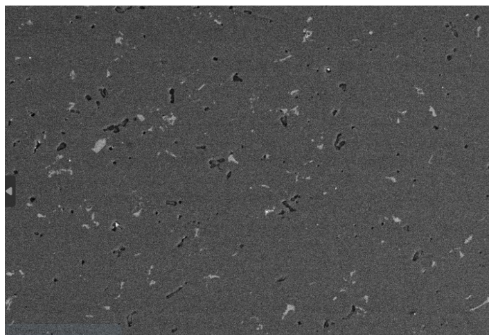
FIGURE 3. SEM image of AA7075 alloy before severe plastic deformation.
