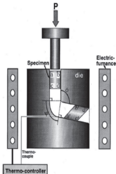
FIGURE 1. Schematic view of the equal channel angular pressing method
